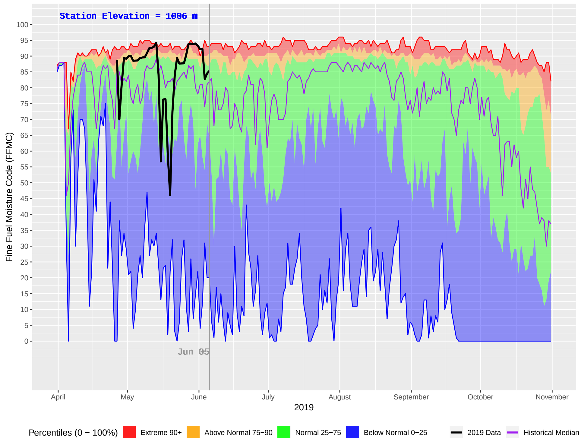
BENSON (228) : Historical (1987–2018) and Current (2019) Daily Fine Fuel Moisture Code (FFMC)
