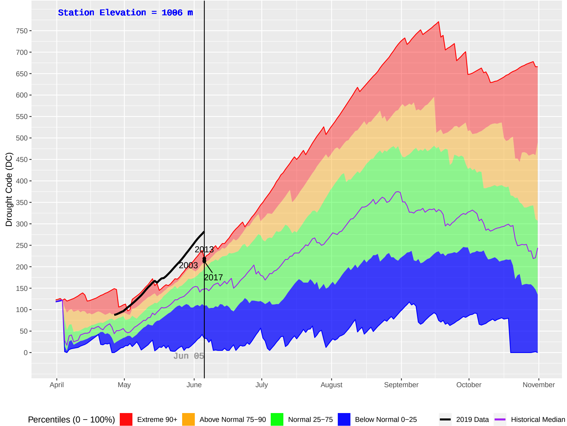
BENSON (228) : Historical (1987–2018) and Current (2019) Daily Drought Code (DC)
