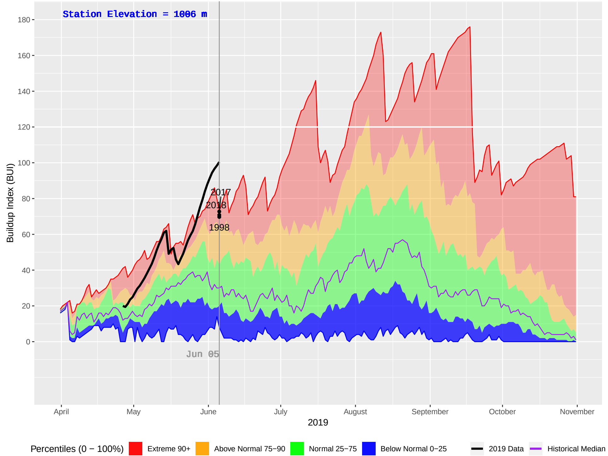
BENSON (228) : Historical (1987–2018), Current (2019) Daily Buildup Index (BUI)
