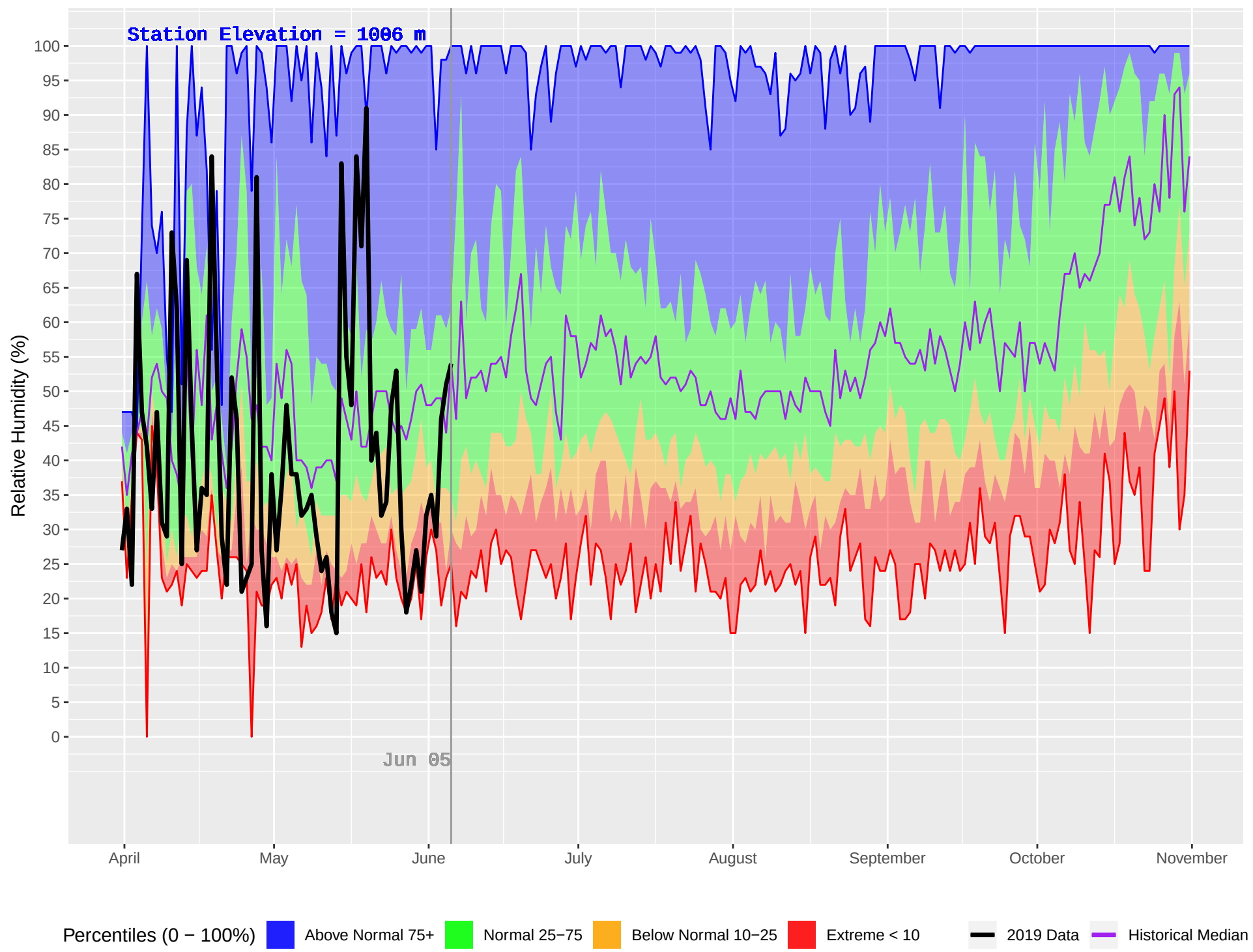
BENSON (228) : Historical (1987–2018) and Current (2019) Daily Relative Humidity
