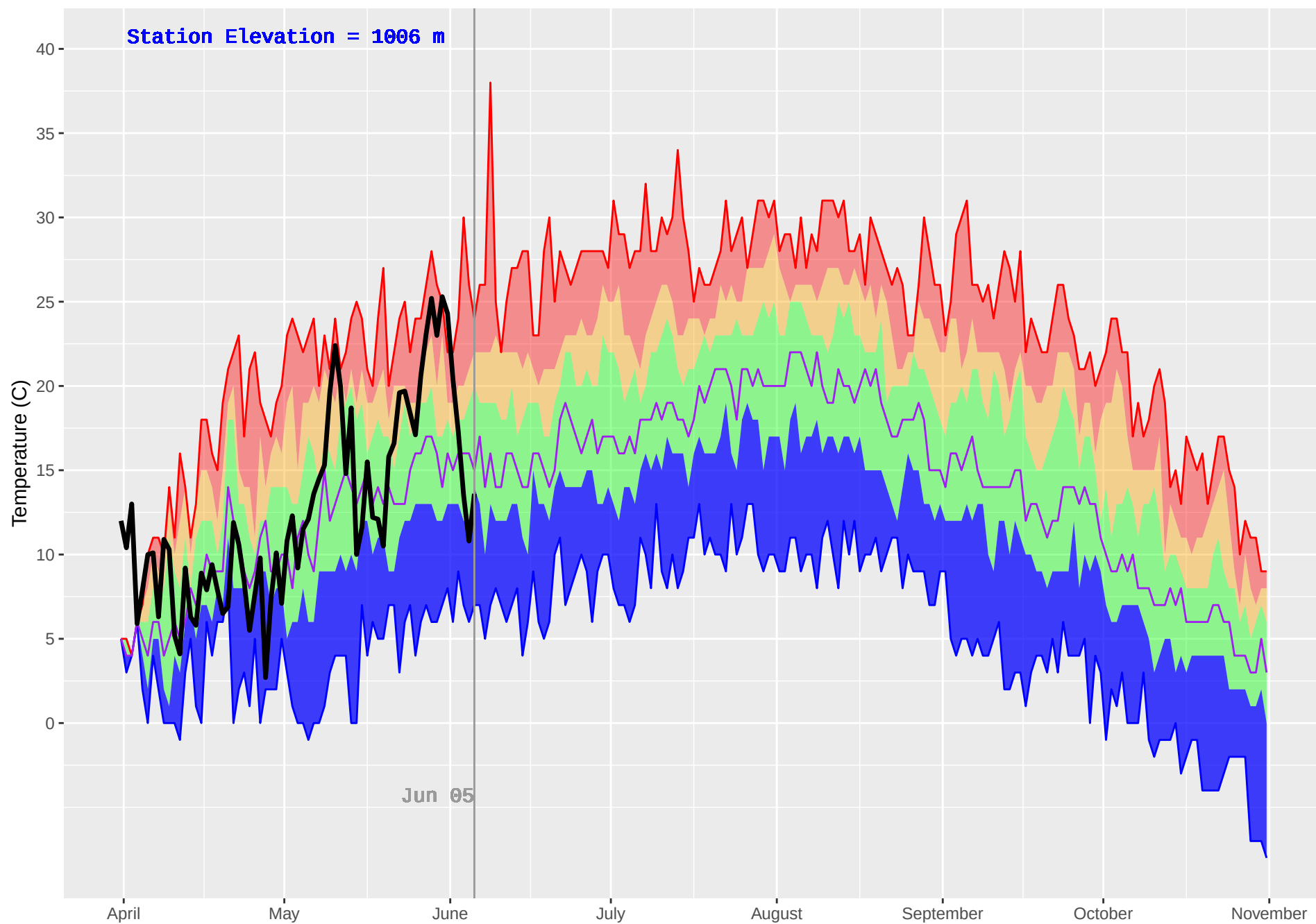
BENSON (228) : Historical (1987–2018) and Current (2019) Daily Temperature
