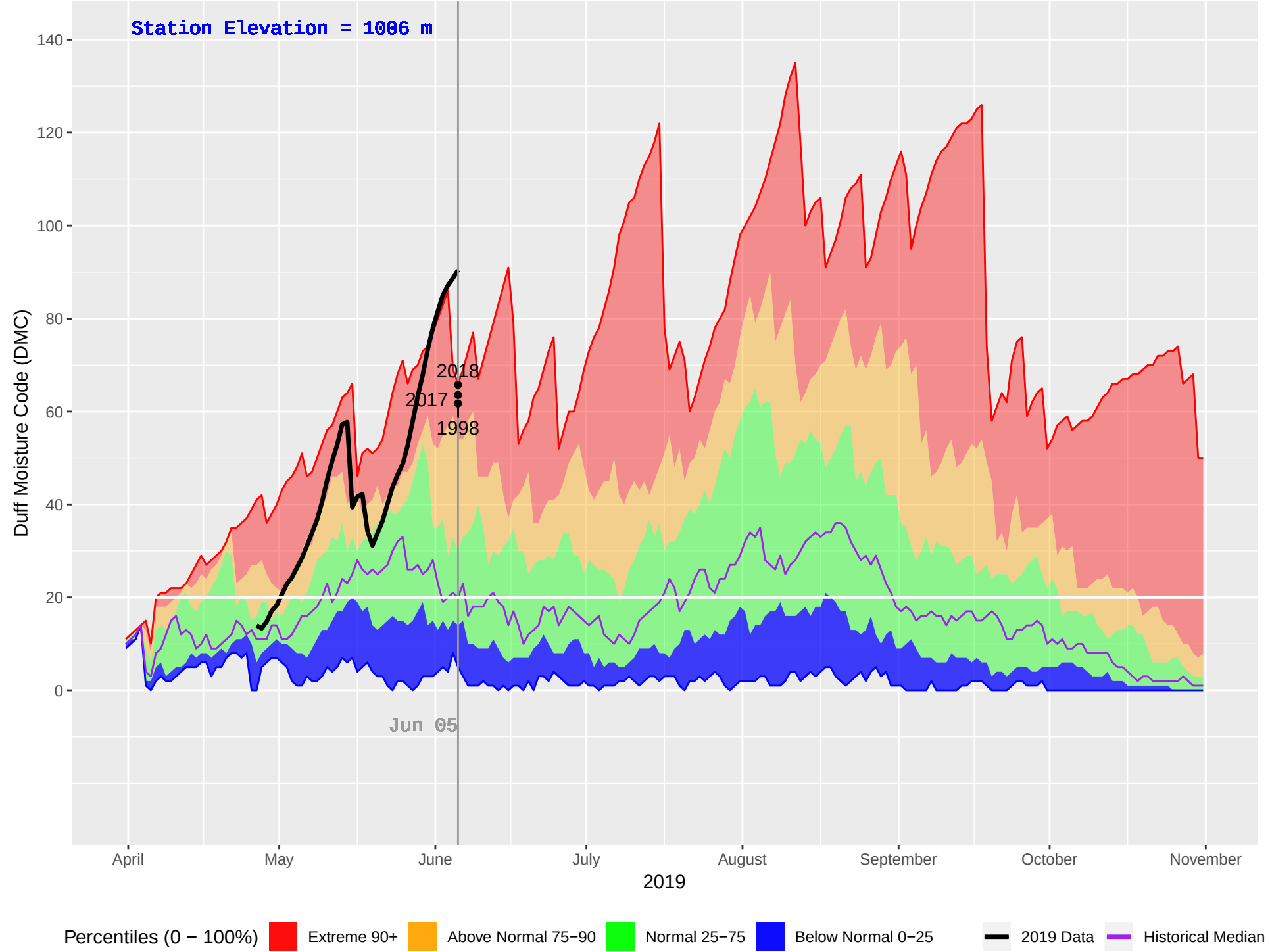
BENSON (228) : Historical (1987–2018), Current (2019) Daily Duff Moisture Code (DMC)
